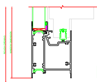
201 SILL SERIES: 3500
